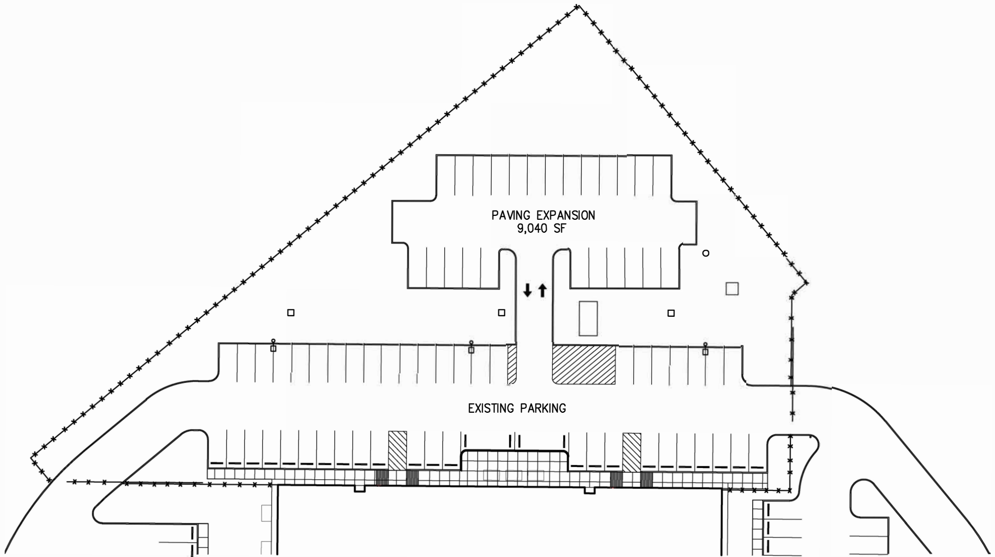
NORTH ANNEX PARKING EXPANSION
